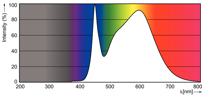
LEDtube HF 1200mm SO 16.5 W /840 T8
