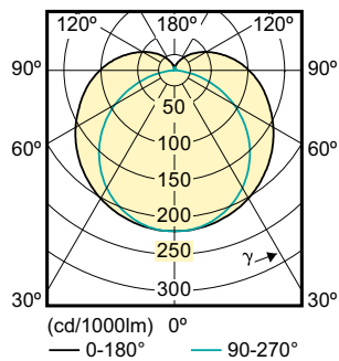
LEDtube HF 1200mm SO 16.5 W T8
