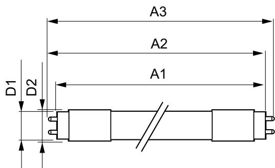
LEDtube HF 1200mm SO 16.5W 840 T8
