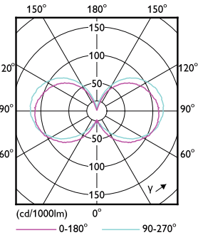
LEDbulb CLA WGD CRI90
